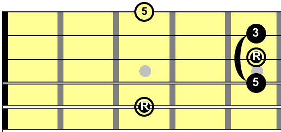
Pattern 2 (A-form)
